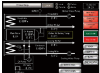
Operation interface
