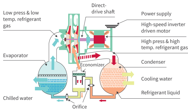
Centrifugal two-stage compressor
